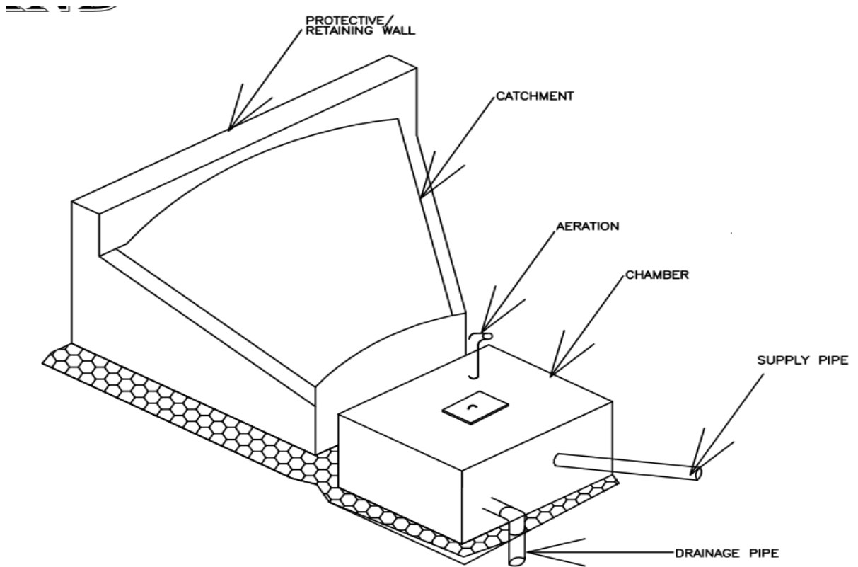
PERSPECTIVE VIEW
